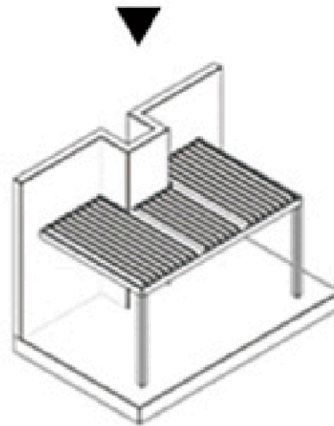
MULTI-WALL INSTALLATION
