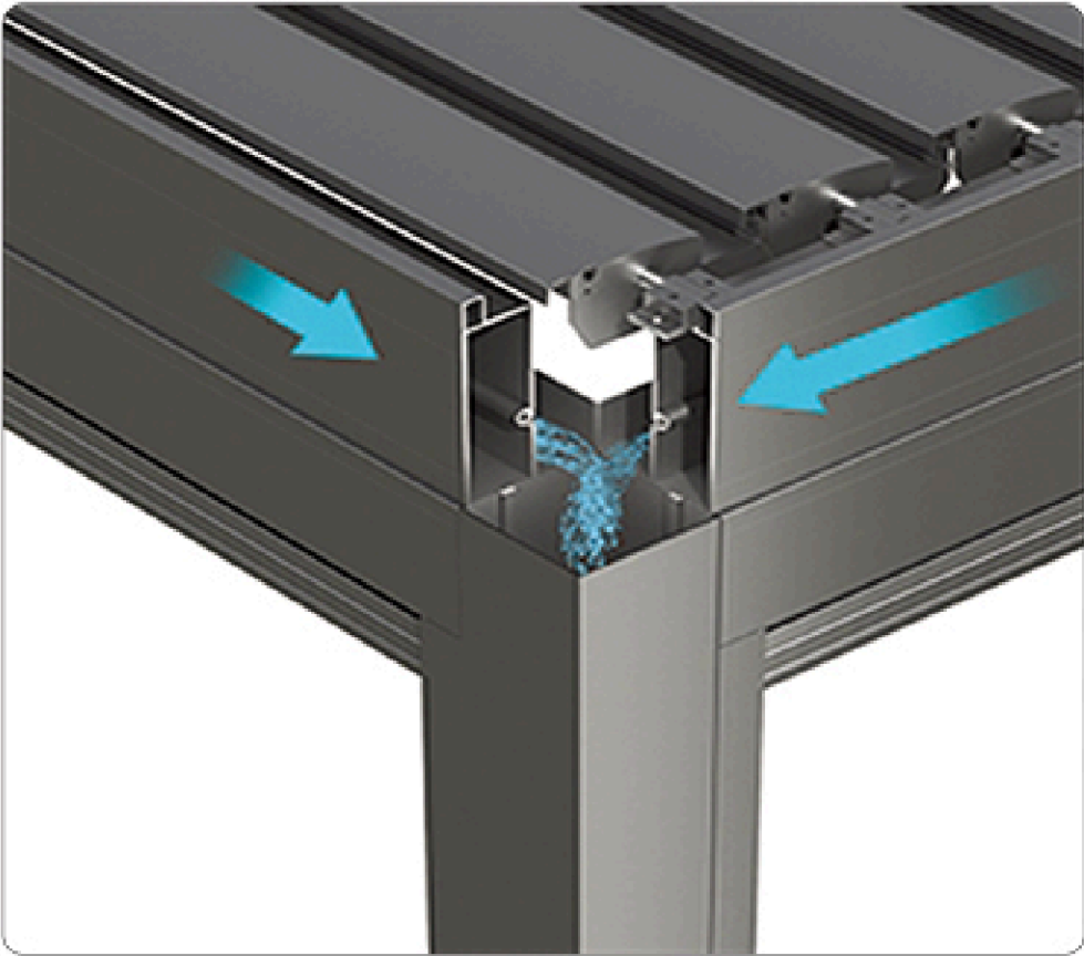
Rainwater direction
