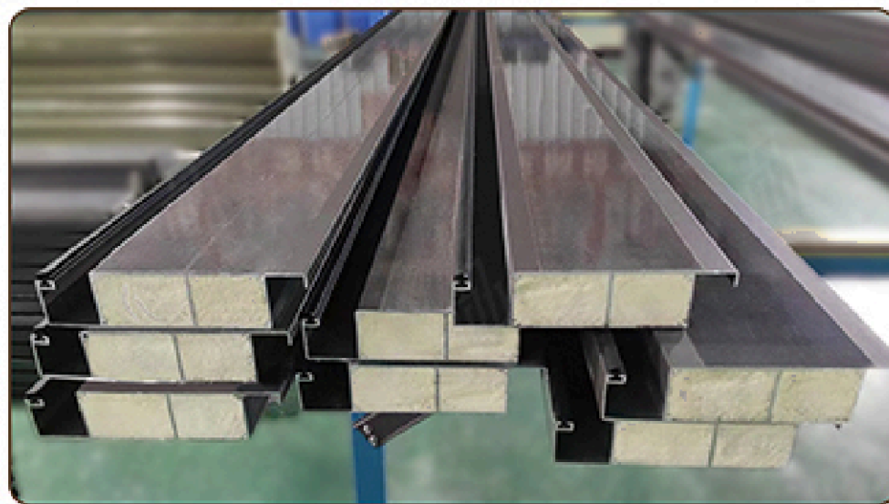
Insulation Foam Added into Louver Blade
